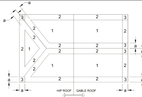
ROOF ZONES FOR GENERIC BUILDING
