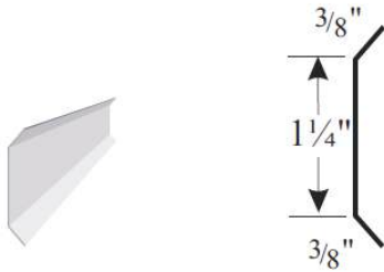
CF1 Counterflashing
